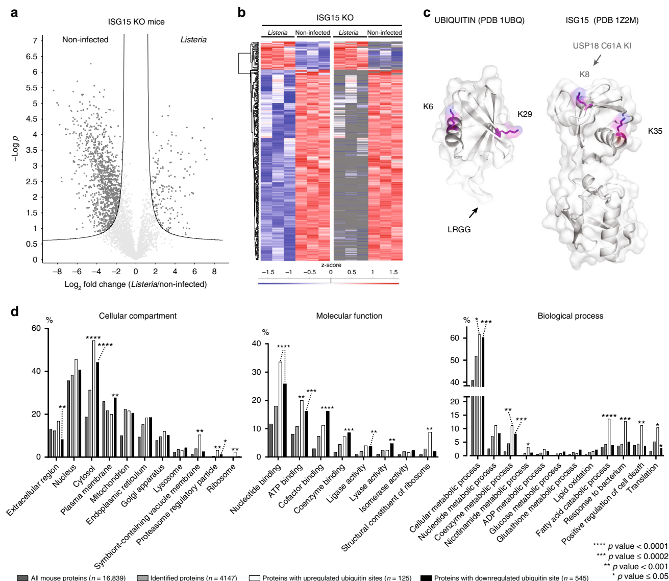
Fig. 3 Loss of ubiquitin sites following infection and evidence for mixed ISG15/Ubiquitin chains. a Volcano plot showing significantly regulated ubiquitin sites upon Listeria infection of Isig15 -/- animals. The fold change (in \log_2 ) of each GlyGly(K) site is shown on the x-axis, while the statistical significance ( -\log P -value) is shown on the y-axis. In total, 168 GlyGly(K) sites were significantly upregulated during infection, while 1138 sites were downregulated (Supplementary Data 3). b Heatmap representation of significantly up- and downregulated ubiquitin sites after non-supervised hierarchical clustering. On the right side, the heatmap is shown with missing values in gray (Supplementary Data 4). c Crystal structures of ubiquitin and ISG15 with modified lysines highlighted. K6 and K29 of ubiquitin are modified following bacterial infection in wild-type animals. K35 of ISG15 is modified following bacterial infection in wild-type animals, and K8 is modified following infection in USP18 C61A/C61A animals. d GO cellular compartment analysis of ubiquitylated proteins (clusters 3 and 4) relative to all proteins identified in the analysis (light gray) and all mouse proteins in the Uniprot/Swiss-Prot database (dark gray). Bars correspond to the percentage of proteins annotated with each GO term. Asterisks indicate significant enrichment relative to the number of identified proteins (two-sided Fisher's exact test).
