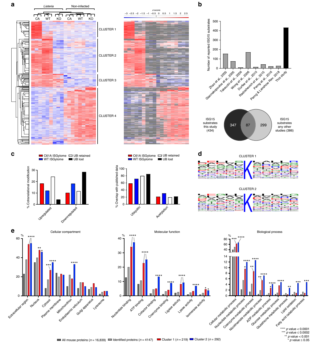
Fig. 2 Identification of in vivo ISGylation sites during Listeria infection. a Heatmap showing significantly regulated GlyGly(K) sites after non-supervised hierarchical clustering. On the right side, the heatmap is shown with missing values in gray. Four major clusters can be observed corresponding to ISG15 sites (clusters 1 and 2) and ubiquitin sites (clusters 3 and 4). b Bar chart and Venn diagram showing the number and overlap of ISGylated proteins identified in this study and previous studies. c Percent of modified proteins from each cluster that are also upregulated following infection according to the shotgun data from liver tissue prior to diglycine enrichment; Percent of modified sites from each cluster that overlap with published ubiquitin or acetylation sites. d Sequence logos were drawn based on the sequence alignment of different ISGylation sites and their + 5 and - 5 flanking regions. e GO analysis of ISGylated proteins (clusters 1 and 2) relative to all proteins identified in this analysis (gray) and all mouse proteins in the Uniprot/Swiss-Prot database (black). Bars correspond to the percentage of proteins annotated with each GO term. Asterisks indicate significant enrichment relative to the number of identified proteins (two-sided Fisher's exact test).
