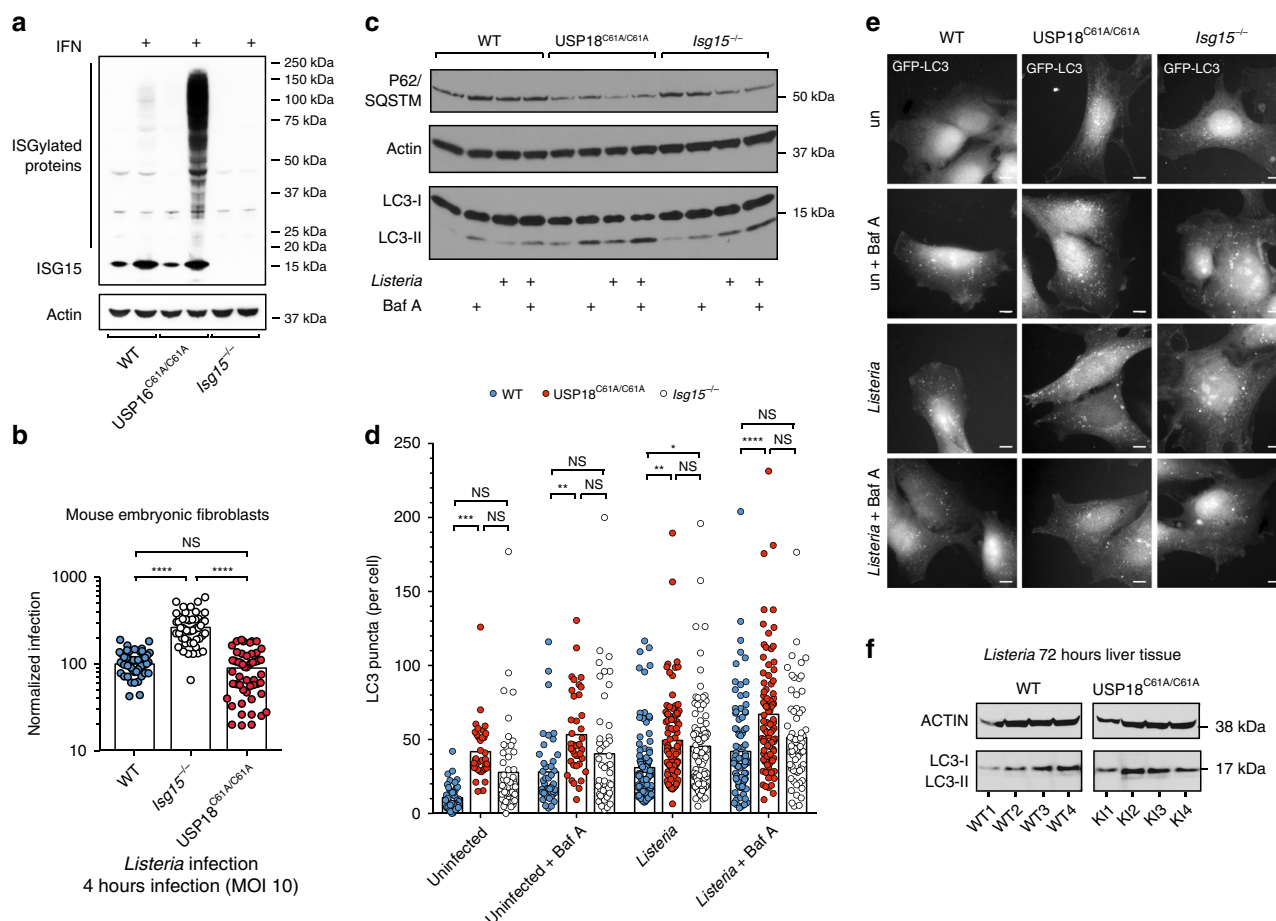
Fig. 5 ISGylation alters basal and infection-induced autophagy. a SDS-PAGE of wild-type, USP18 C61A/C61A , and lsg15 -/- mouse embryonic fibroblasts treated with interferon \beta (1000 units/mL for 24 h), bottom ISG15 blot is a short exposure of the upper panel. b Mouse embryonic fibroblasts MEFs (wild-type, lsg15 -/- KO, and USP18 C61A/C61A KI) were infected with Listeria monocytogenes strain EGD for 4 h at an MOI of 10. Cells were lysed, and bacterial CFUs were enumerated through serial dilution. Wild-type values were normalized to 100; data from three independent experiments are shown. Statistical analysis was conducted using one-way ANOVA and Tukey's test post hoc. c SDS-PAGE analysis of wild-type or USP18 C61A/C61A MEFs treated with Bafilomycin A (100 nM for 20 min prior to lysis) at baseline or following 4 h of infection with Listeria at an MOI of 10. Immunoblot is a representative image of five independent experiments. d GFP-LC3 puncta per cell; data shown are compiled from four separate experiments WT (un, un + Baf, EGD, EGD + Baf) n = 408, 450, 984, 987 (USP18 C61A/C61A (un, un + Baf, EGD, EGD + Baf) n = 352, 410, 1038, 1014 , lsg15 -/- (un, un + Baf, EGD, EGD + Baf) n = 183, 224, 710 , and 470 individual cells per condition were enumerated). Statistical analysis was conducted using one-way ANOVA and Tukey's test post hoc (exact p -values (Supplementary Fig. 4b). NS nonsignificant, * p < 0.05 ; ** p < 0.01 ; *** p < 0.001 ; **** p < 0.0001 . e Representative images of cells stably expressing GFP-LC3 and treated as above with Bafilomycin A or infected with Listeria and treated with Bafilomycin A, scale bar is 5 \mu m. f SDS-PAGE of liver homogenate from n = 4 individual animals either wild-type or USP18 C61A/C61A infected with 5 \times 10^5 Listeria , organs harvested following 72 h of infection. Raw data are available in the source data file.
